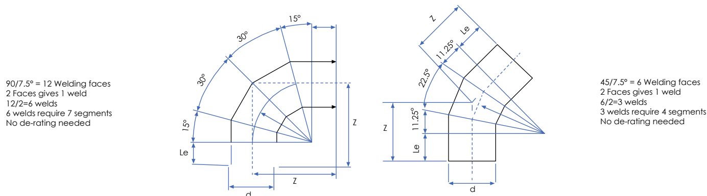
FIGURE 4.15: SEGMENTED BENDS
