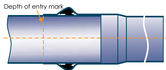
FIGURE 6.4: JOINING OF PVC PIPES
