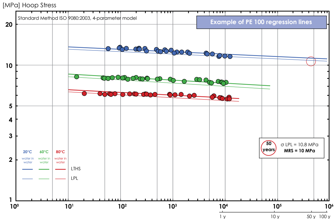
FIGURE 4.2: REGRESSION CURVE OF A MODERN PE 100 MATERIAL
