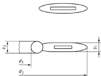
Figure A.1 — Typical steel core gasket design
