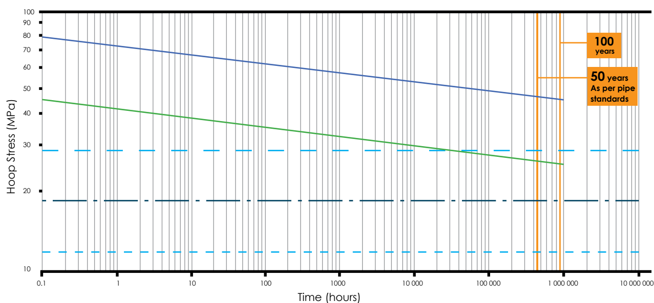
Stress - Time lines for PVC-O, PVC-M and PVC-U
