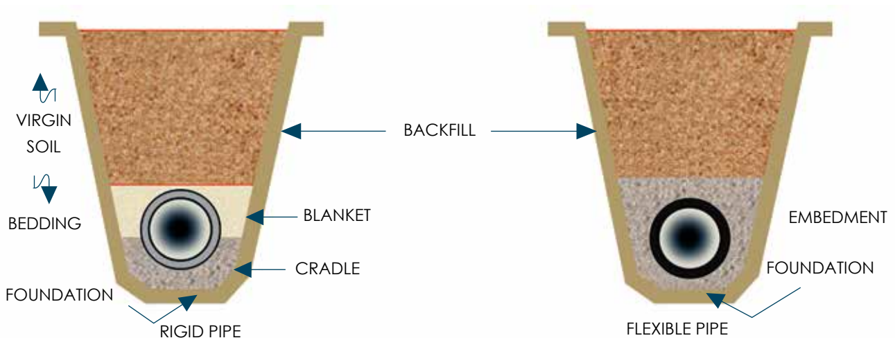
FIGURE 2.10: COMPARISON OF RIGID AND FLEXIBLE PIPE INSTALLATION DETAILS
