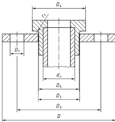
Figure 2 — Socket fusion systems
