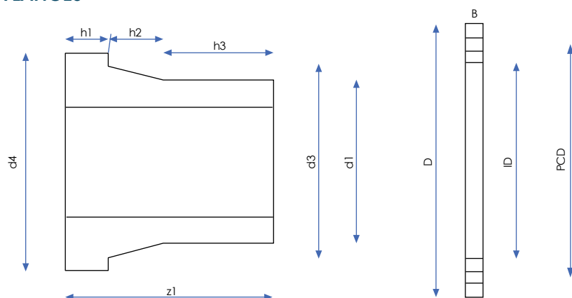
FIGURE 4.12: STUB FLANGES
