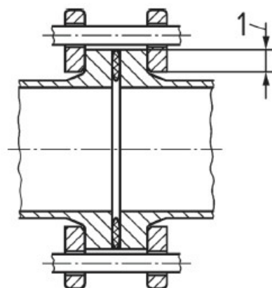
Figure B.1 — Contact area
