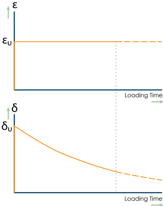
FIGURE 3.7: STRESS RELAXATION OF A PLASTIC MATERIAL UNDER CONSTANT STRESS
