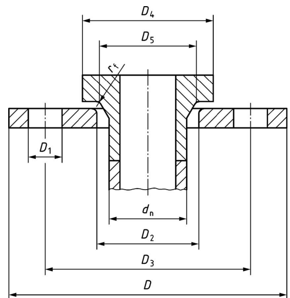
Figure 1-Butt fusion System
