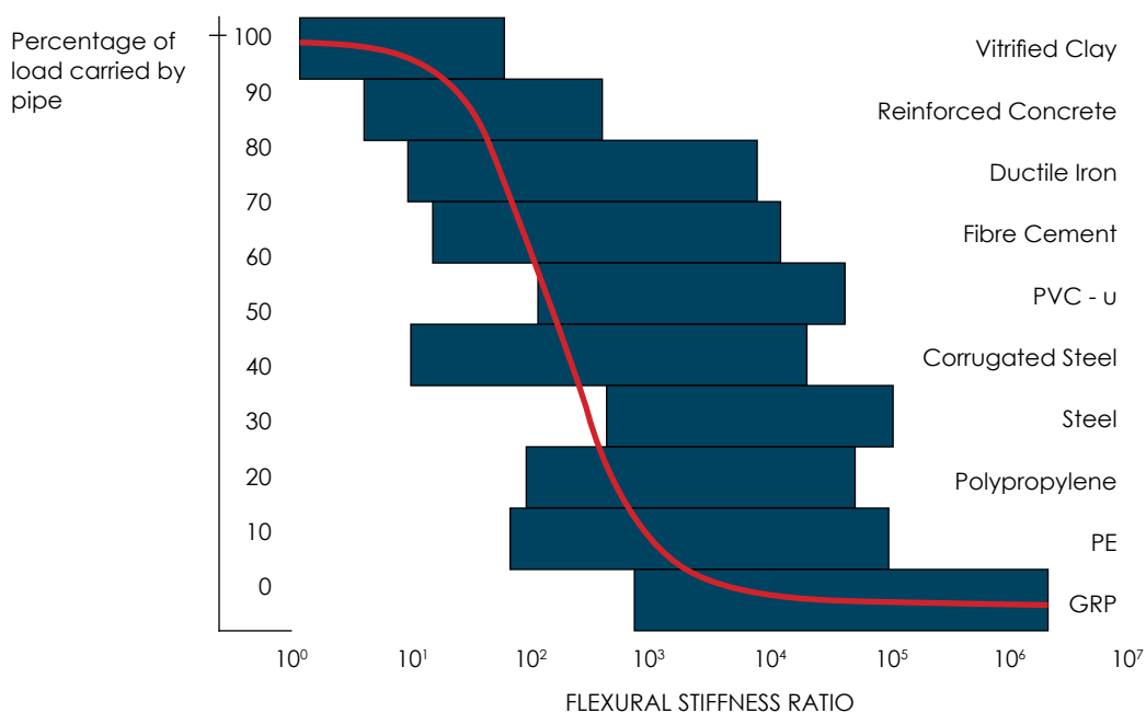
FIGURE 2.2: RANGE OF FLEXURAL STIFFNESS RATIOS FOR PIPE MATERIALS USED IN SOUTH AFRICA
