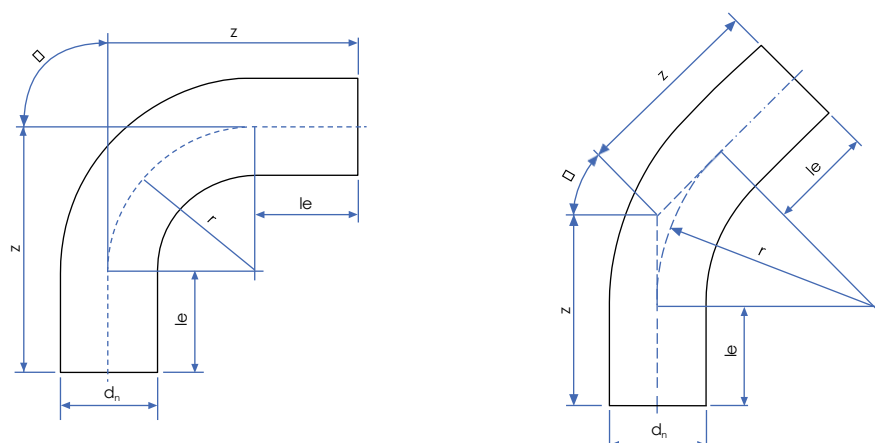
FIGURE 4.16: SEAMLESS BENDS
